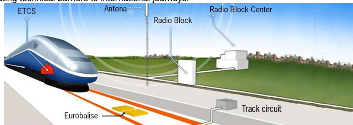
ERTMS components
